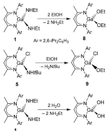
Scheme 3. Synthesis of compounds 8 , 9 , and LGa(OH) 2 .
