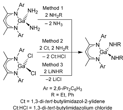
Scheme 1. Methods 1–3 used for the preparation of compounds 1–4 .
