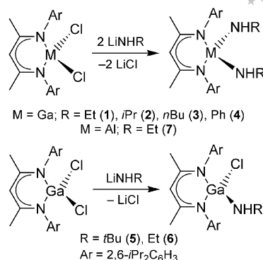
Scheme 2. Synthesis of compounds 1–7 .
